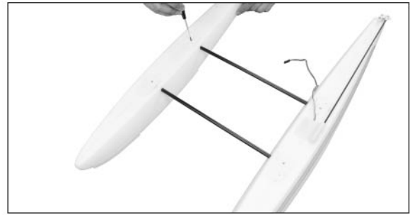
18 Fix glass fibre tubes with PA2.3*20mm screws.
