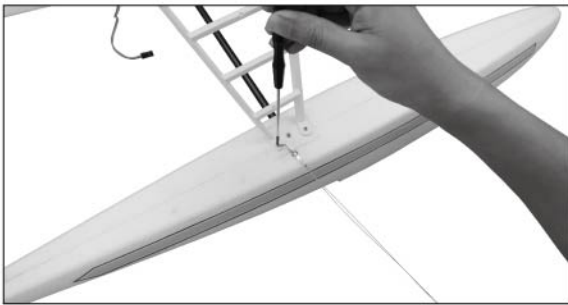
19 Fasten the brackets to the floats with PA2.5*8mm screws.
